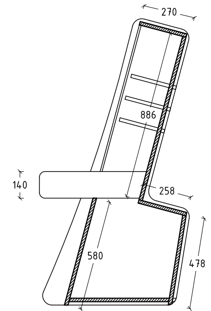
SIDE SECTION
